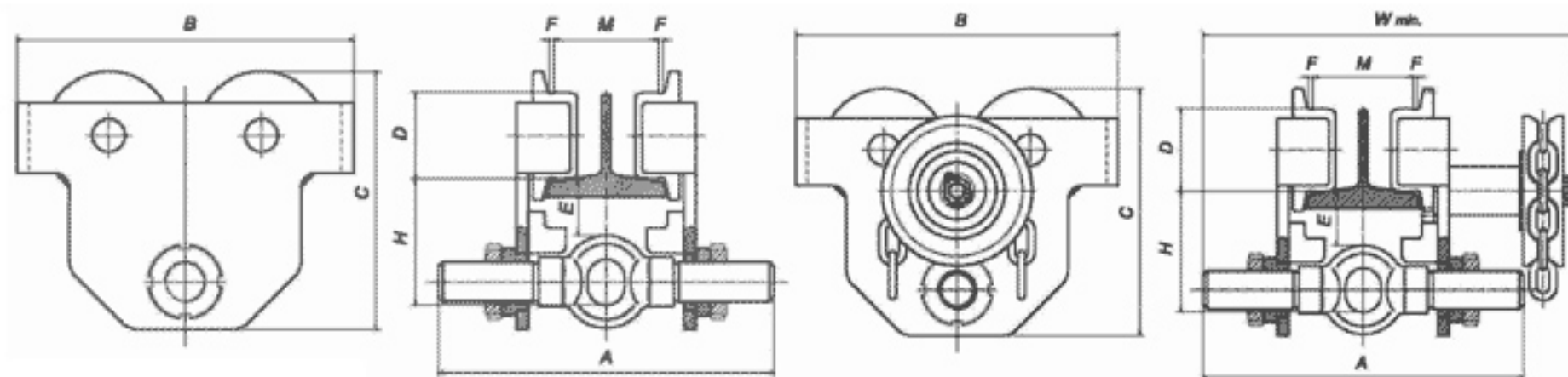
SPT - Type Geared Trolley
